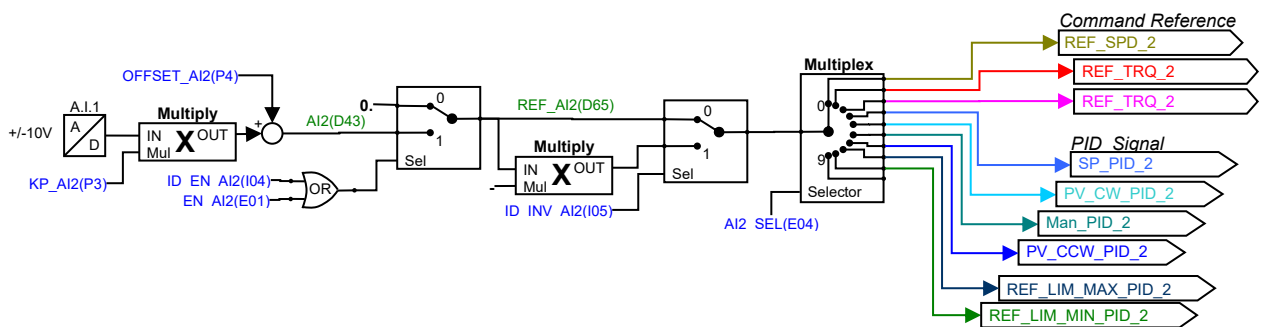
Figure 3: Analog input 2
