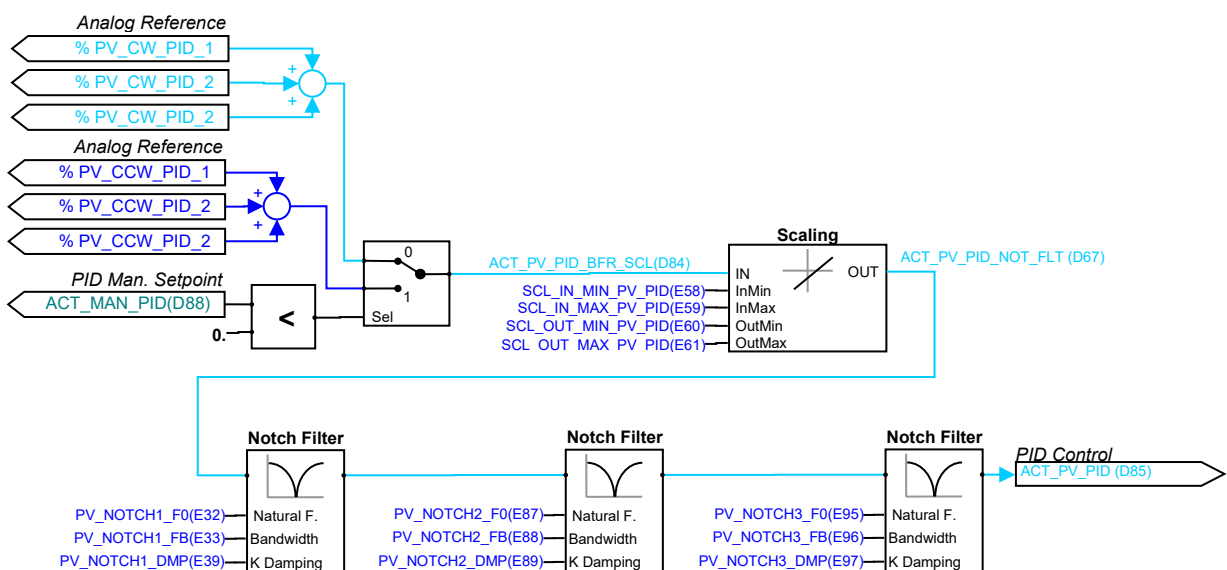
Figure 9: PID Feed-back
