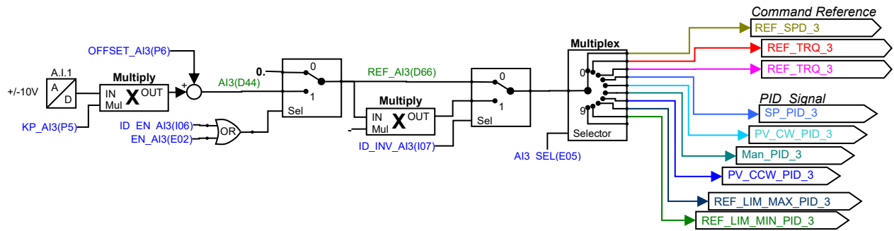
Figure 4: Analog input 3
