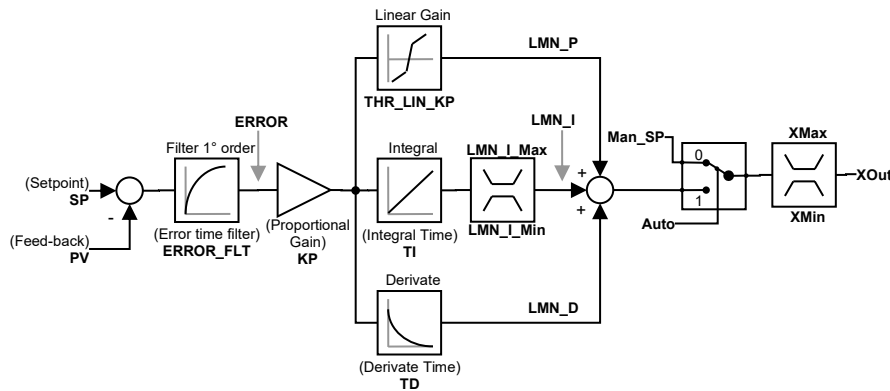
Figure 16: PID function
