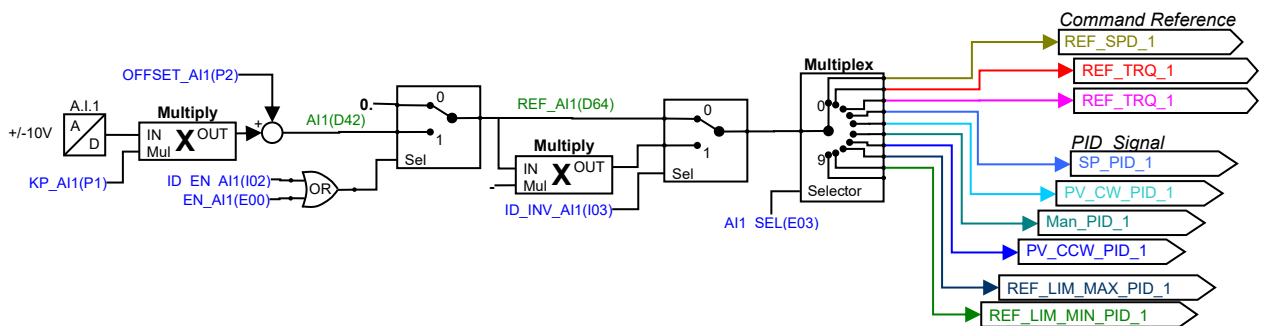
Figure 2: Analog input 1
