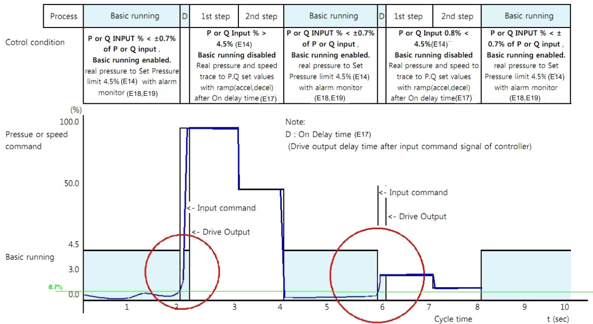
TIMING CHART OF BASIC RUNNING
